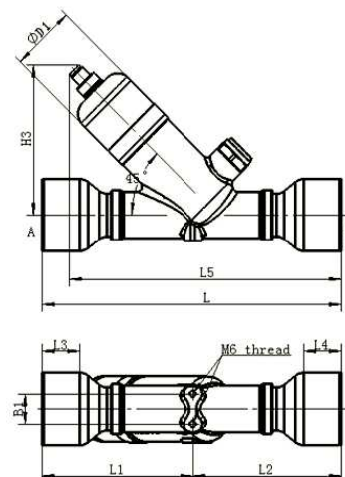
Valve Body - With sight glass: VPF400
