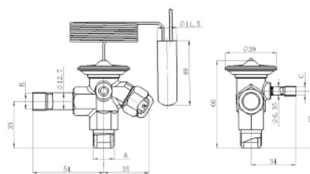
Valve Body - Connection Type: flare/solder/solder
