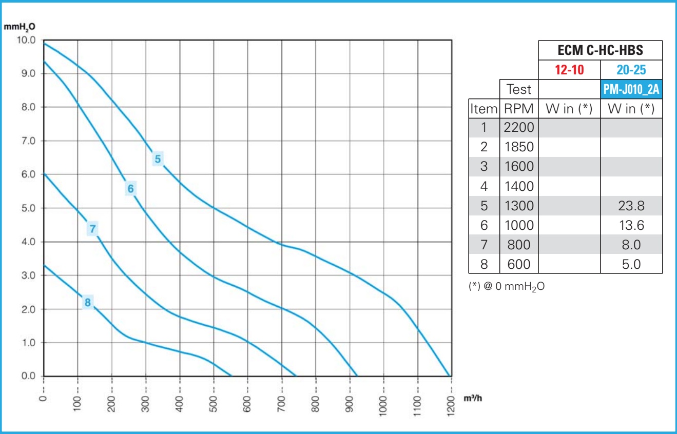
Fan blade air performance curves Ø 300x22°
